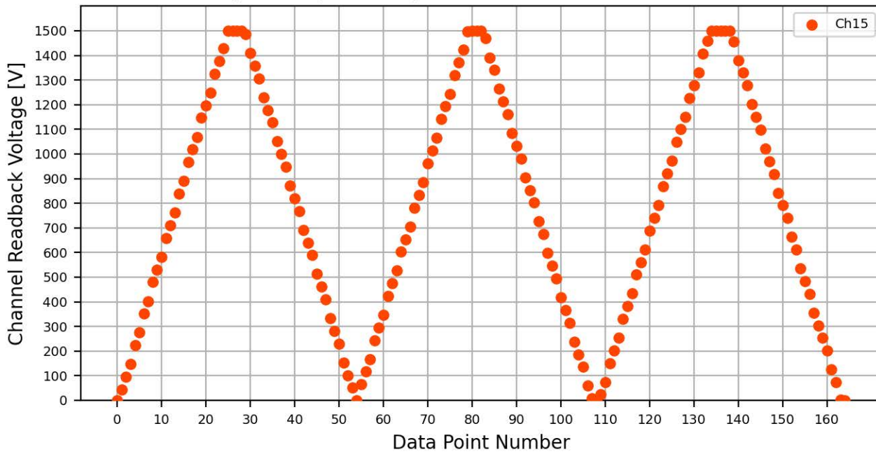
Voltage Ramp Test (Python) Bd #094, Slot #2, Ch #15
