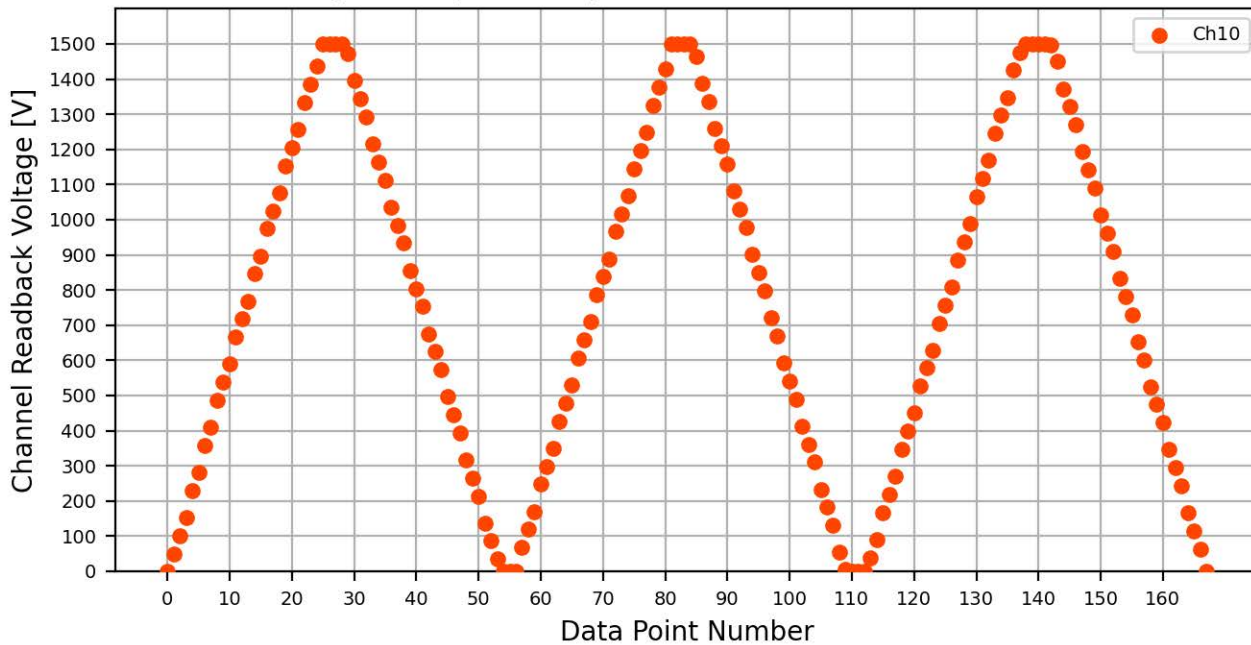
Voltage Ramp Test (Python) Bd #094, Slot #2, Ch #10
