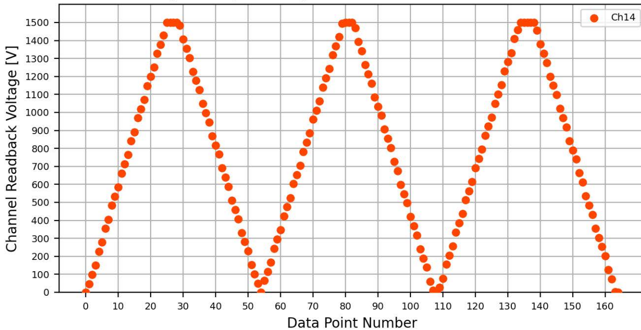
Voltage Ramp Test (Python) Bd #094, Slot #2, Ch #14
