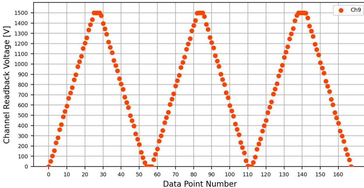
Voltage Ramp Test (Python) Bd #094, Slot #2, Ch #9
