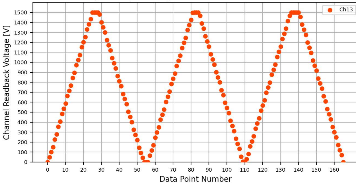
Voltage Ramp Test (Python) Bd #094, Slot #2, Ch #13
