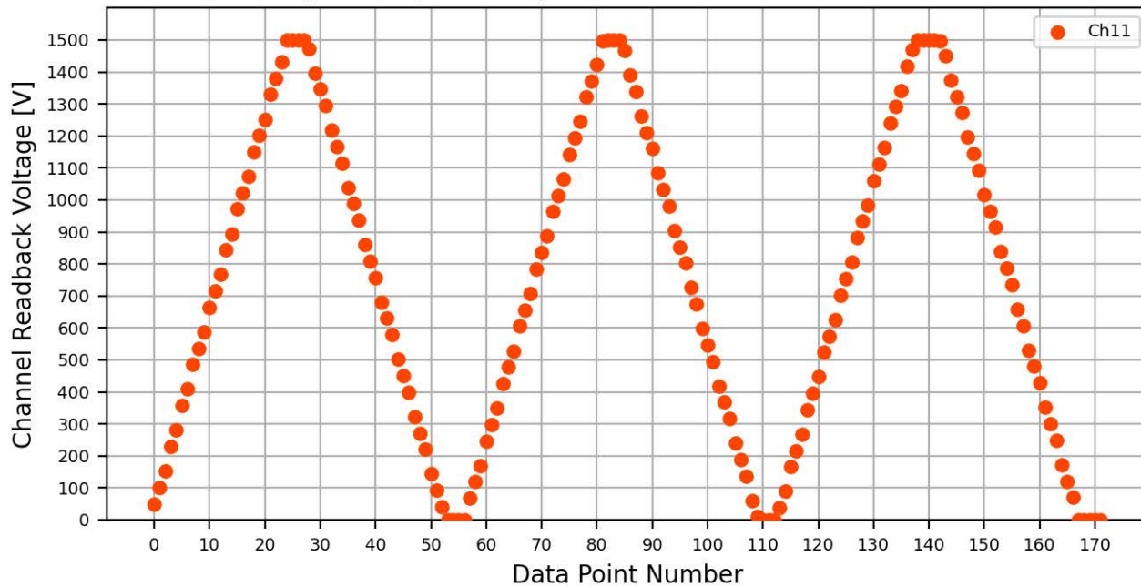
Voltage Ramp Test (Python) Bd #094, Slot #2, Ch #11
