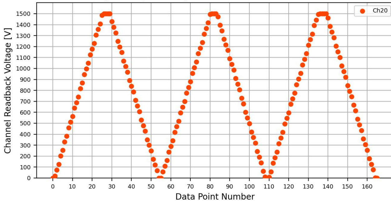
Voltage Ramp Test (Python) Bd #094, Slot #2, Ch #20
