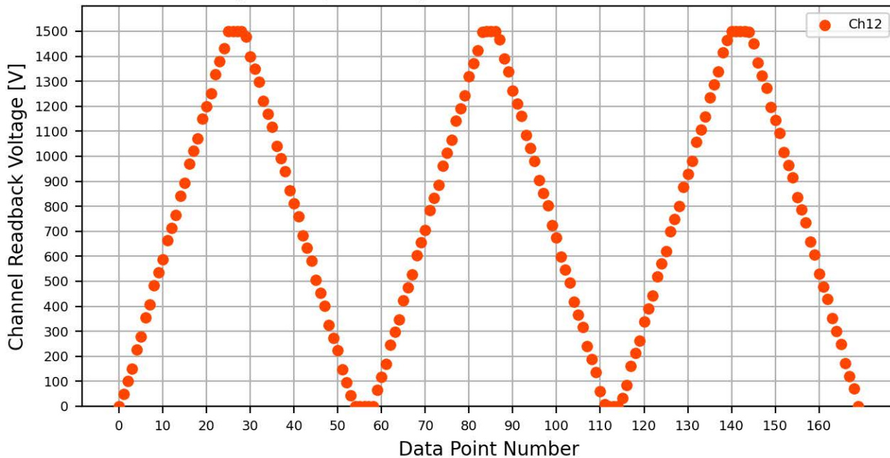
Voltage Ramp Test (Python) Bd #094, Slot #2, Ch #12
