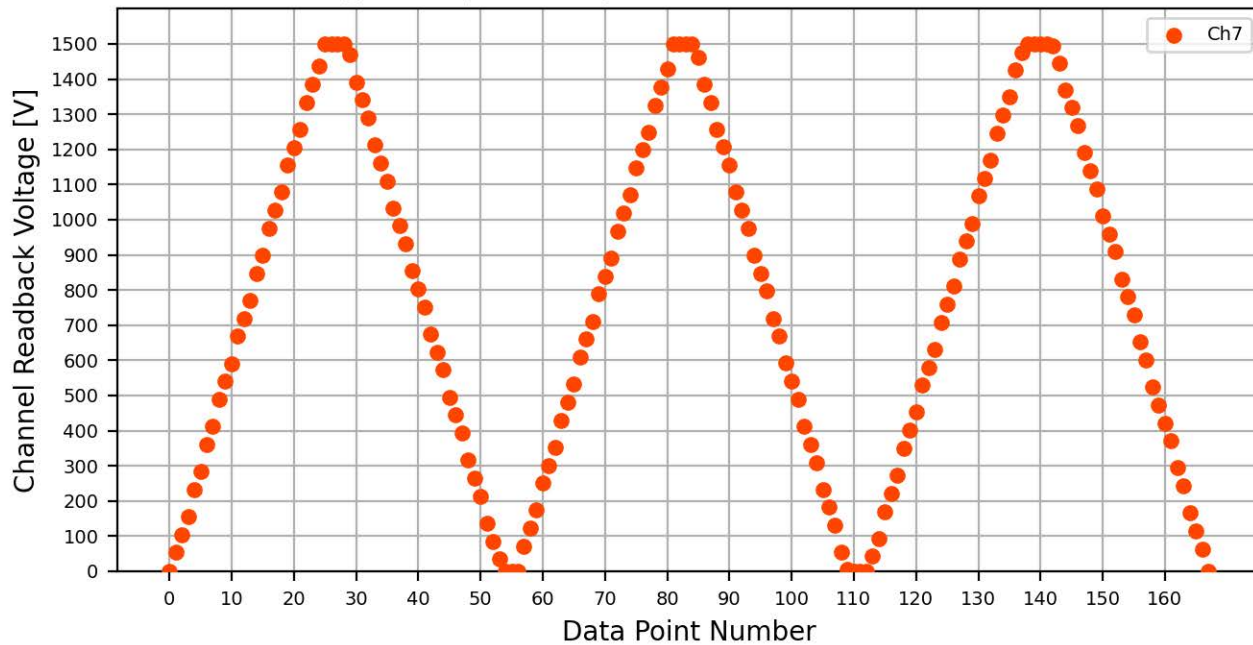
Voltage Ramp Test (Python) Bd #094, Slot #2, Ch #7
