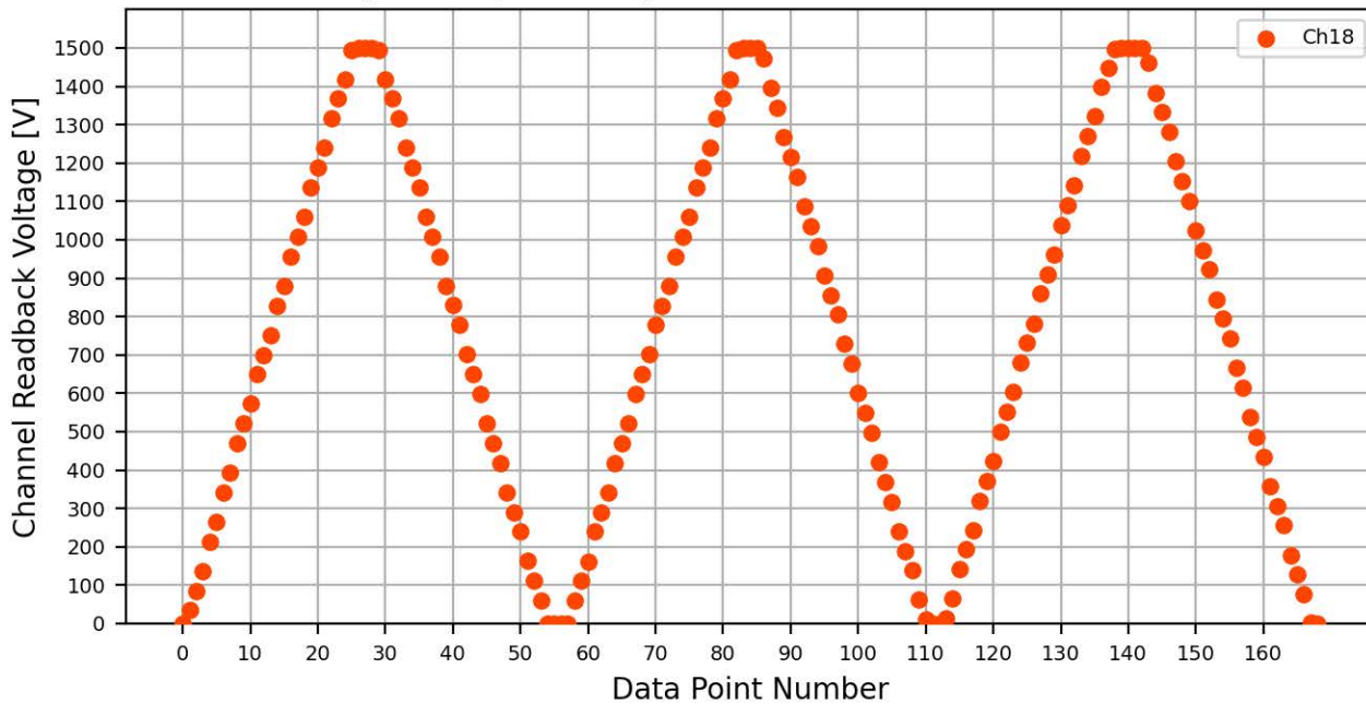
Voltage Ramp Test (Python) Bd #094, Slot #2, Ch #18
