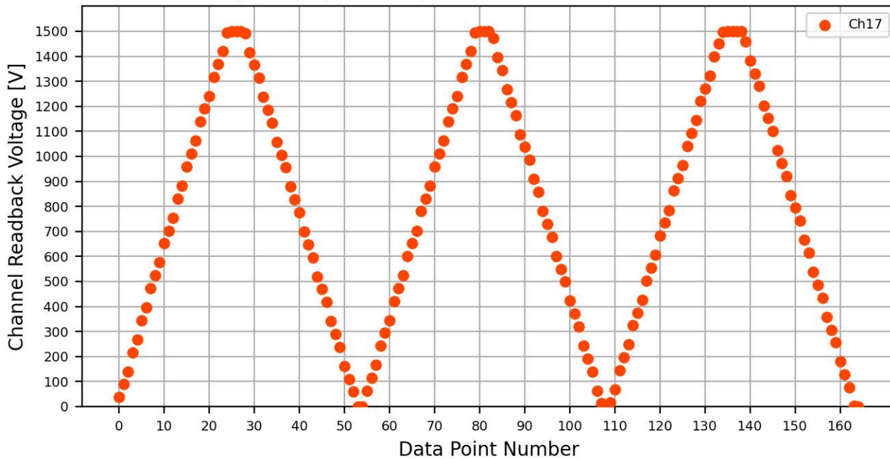
Voltage Ramp Test (Python) Bd #094, Slot #2, Ch #17
