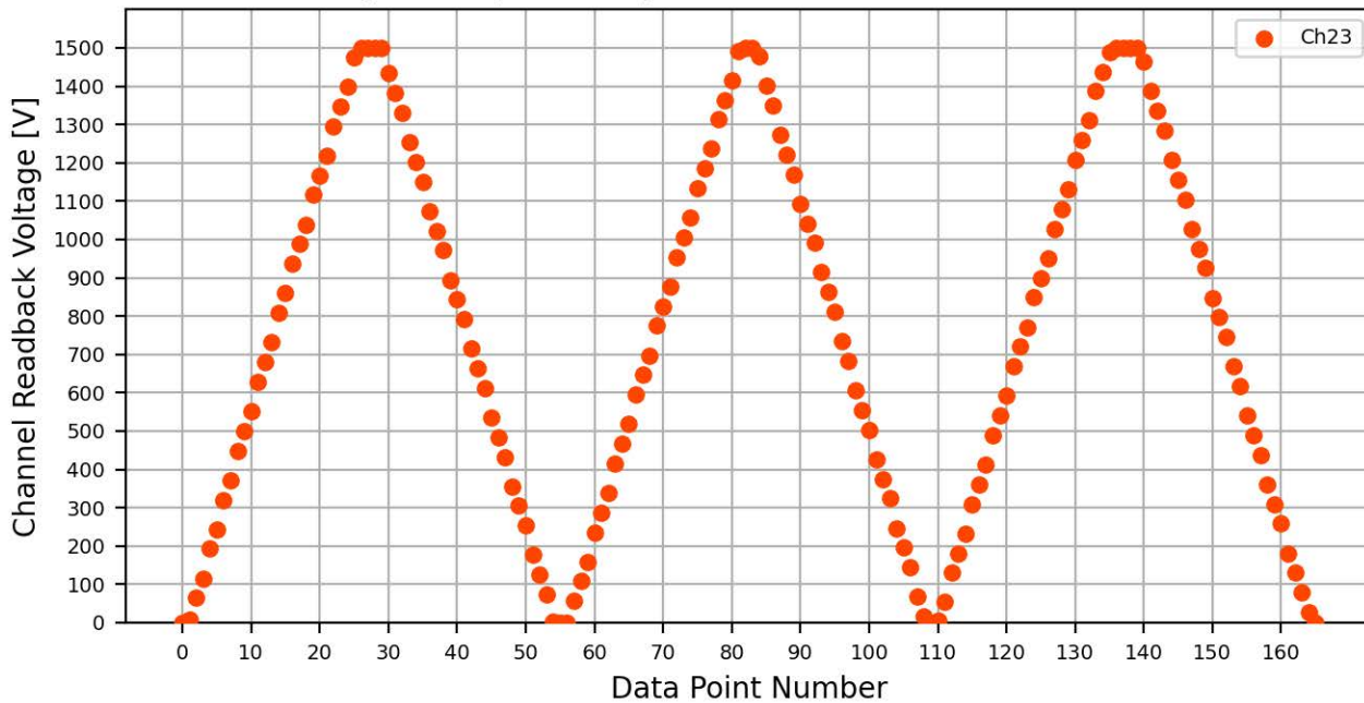
Voltage Ramp Test (Python) Bd #094, Slot #2, Ch #23
