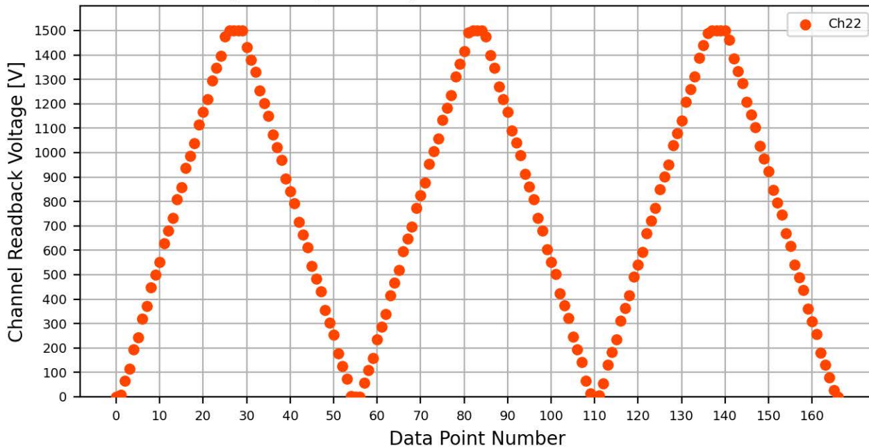
Voltage Ramp Test (Python) Bd #094, Slot #2, Ch #22
