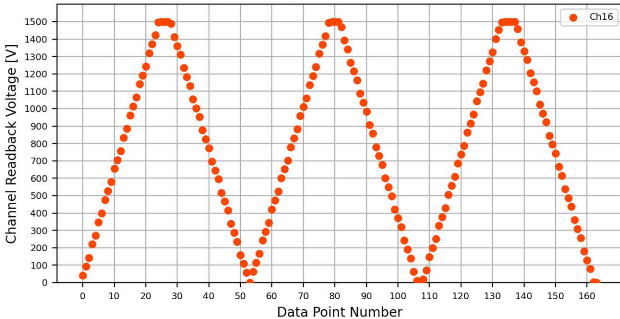
Voltage Ramp Test (Python) Bd #094, Slot #2, Ch #16
