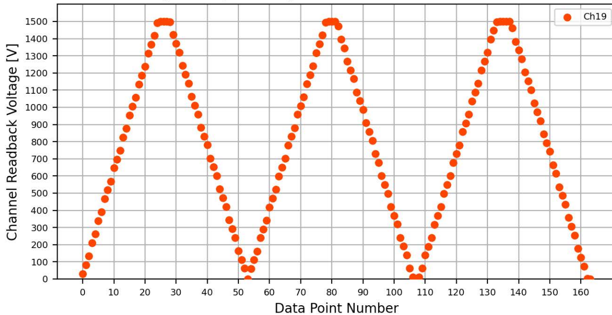
Voltage Ramp Test (Python) Bd #094, Slot #2, Ch #19
