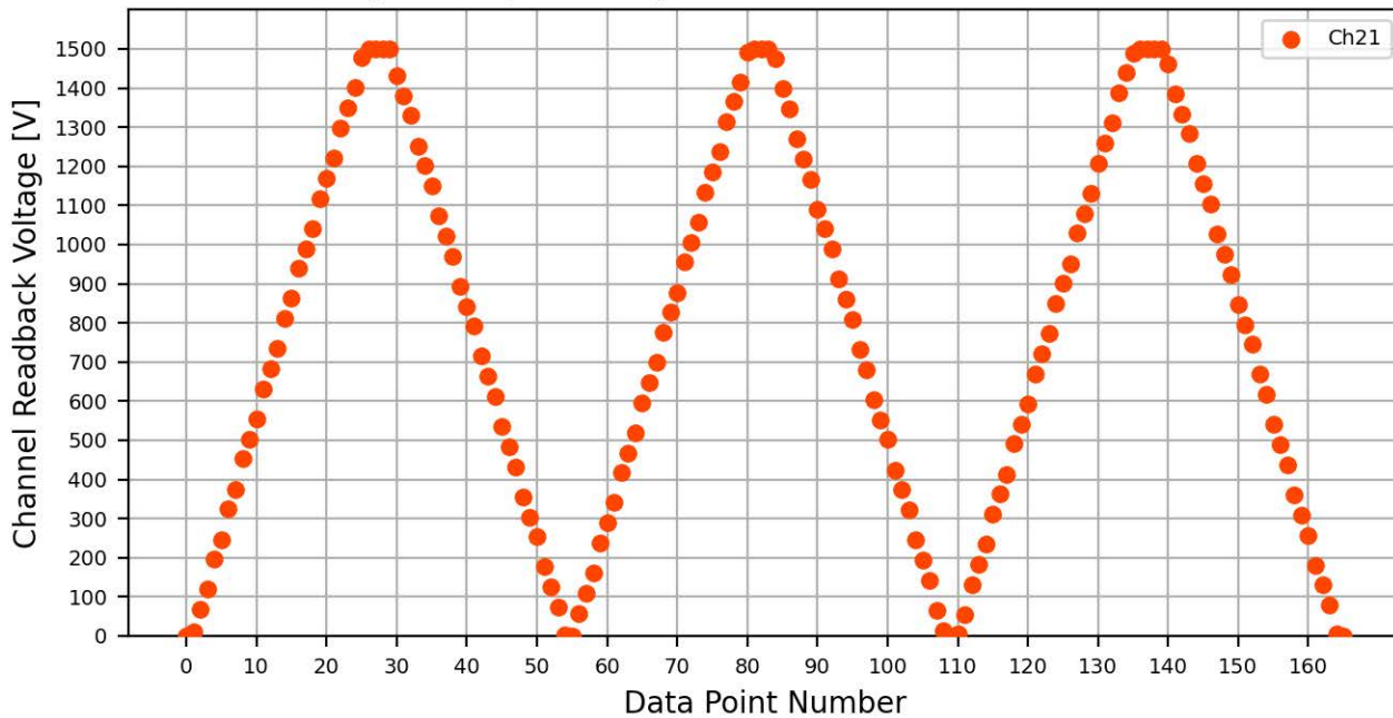
Voltage Ramp Test (Python) Bd #094, Slot #2, Ch #21
