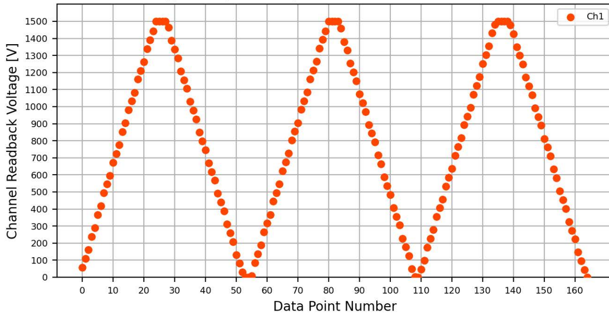
Voltage Ramp Test (Python) Bd #094, Slot #2, Ch #1
